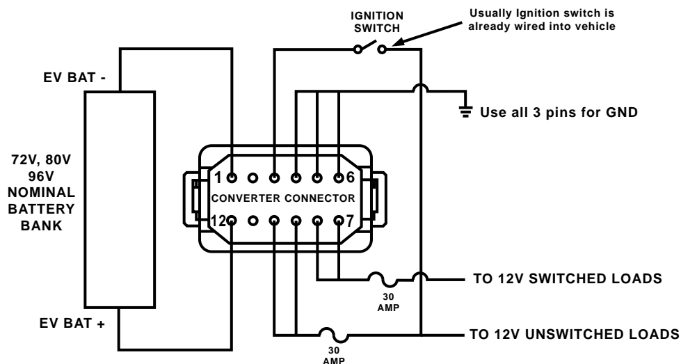
TYPICAL INSTALLATION WITH SWITCHED & UNSWITCHED LOADS (Total load must be less than 30A)
