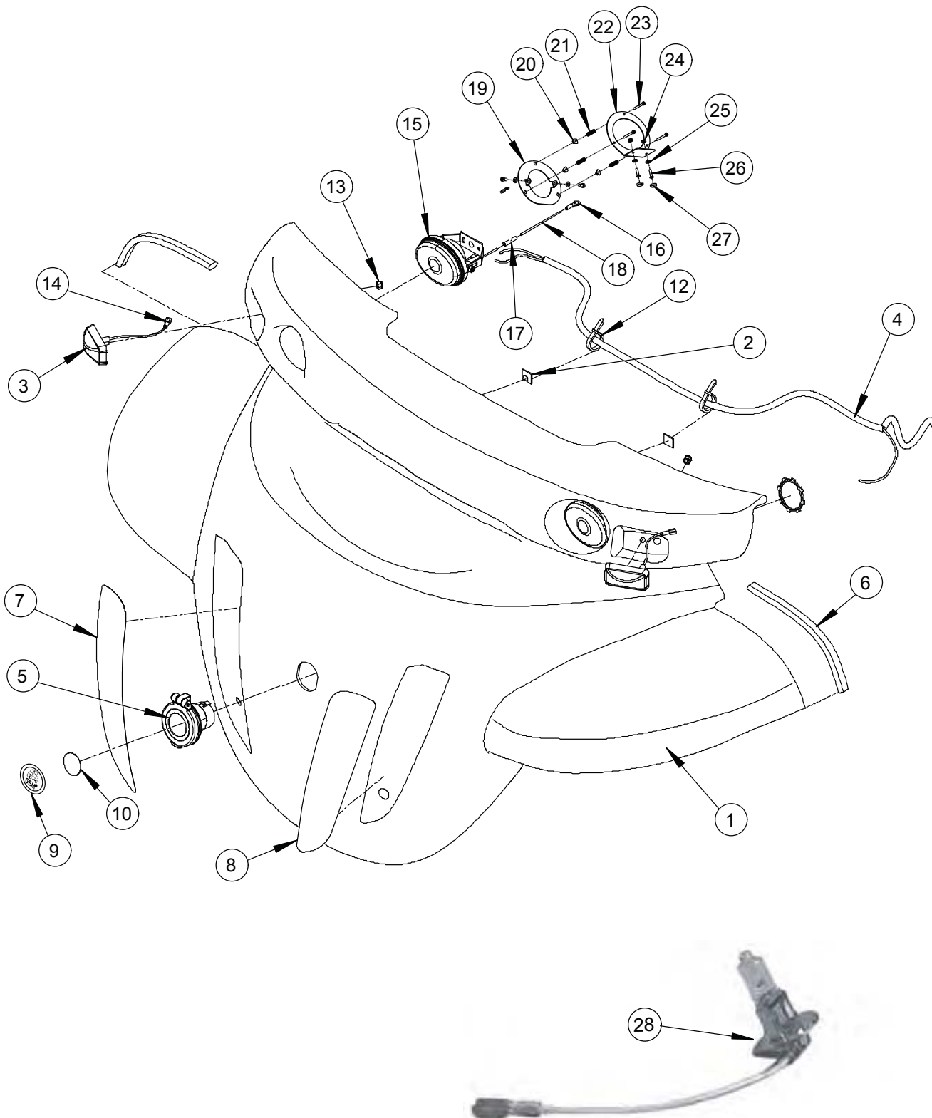
ASSY, HOOD COMPLETE- SEE NEXT PAGE FOR PARTS LISTING
