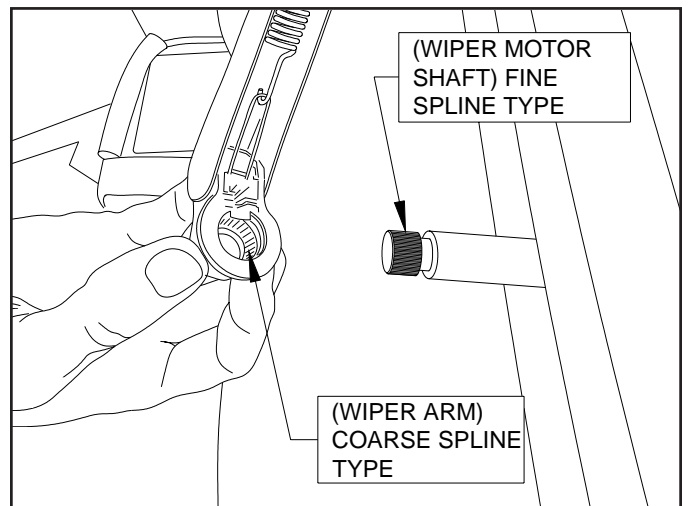
Fig. # 6 Note the mismatched splines
