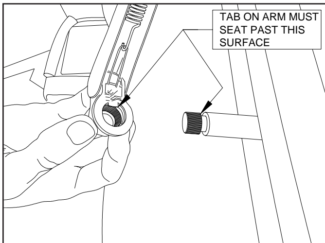
Fig. # 8 Install new wiper assembly to wiper motor shaft
