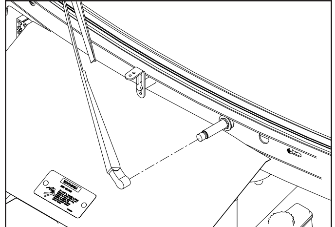
Fig. # 5 Remove wiper arm assembly
